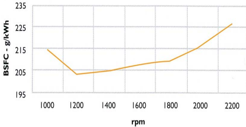
93kW Fuel Consumption
