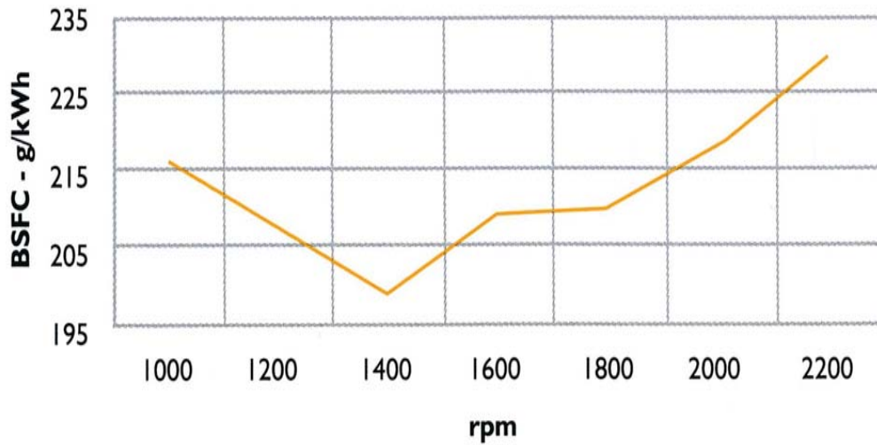
74.2kW Fuel Consumption
